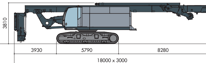
Base carrier with mast without counterweight Carro base con mast senza zavorra ~ 70900 kg
