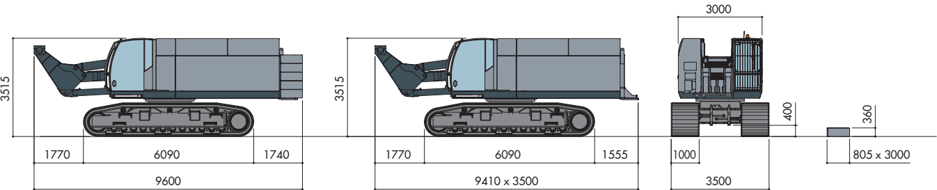
Base carrier complete with counterweight Carro base con zavorra ~ 82200 kg Base carrier without counterweight Carro base senza zavorra ~ 63700 kg Counterweight Zavorra 5x3700 kg (18500 kg)
