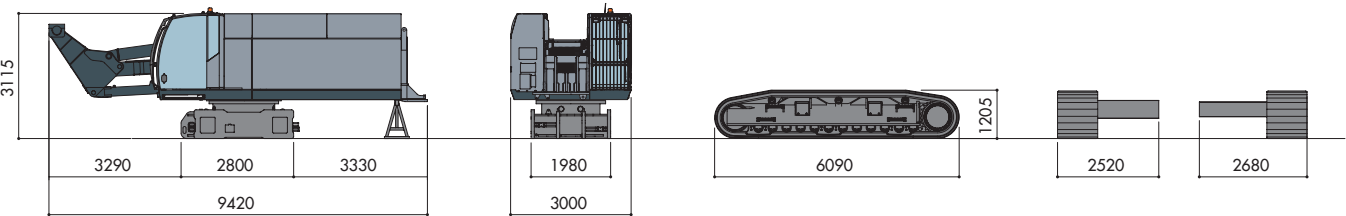
Base carrier Carro base ~ 39700 kg Tracks Cingoli ~ 2x12000 kg
