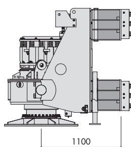
Drilling axis extension Slitta supplementare
