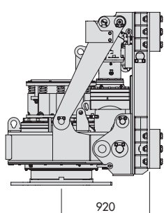
Drilling axis Interasse
