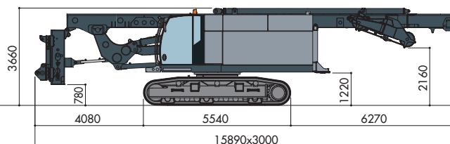
Base carrier with mast without counterweight Carro base con mast senza zavorra ~ 60500 kg
