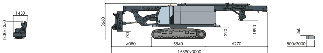
H26 rotary Rotary H26 ~ 4700 kg
