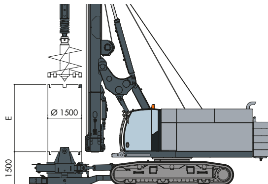
Piling arrangement with crowd winch Allestimento pali con argano pull down
