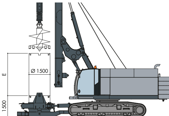
Piling arrangement with crowd ram Allestimento pali con martinetto pull down
