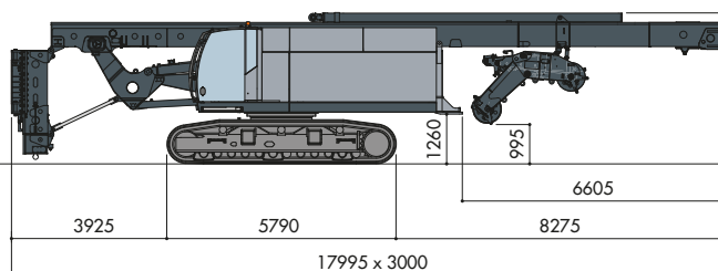
Base carrier with mast without counterweight Carro base con mast senza zavorra ~ 70900 kg
