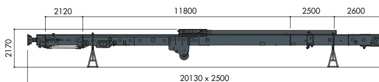
Mast Mast ~ 15600 kg
