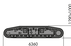
Tracks Cingoli 2 x ~11000 kg
