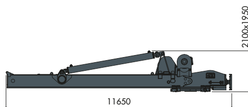
Base mast with pull down and auxiliary winch Mast base con argano pull down e argano ausiliario ~17200 kg
